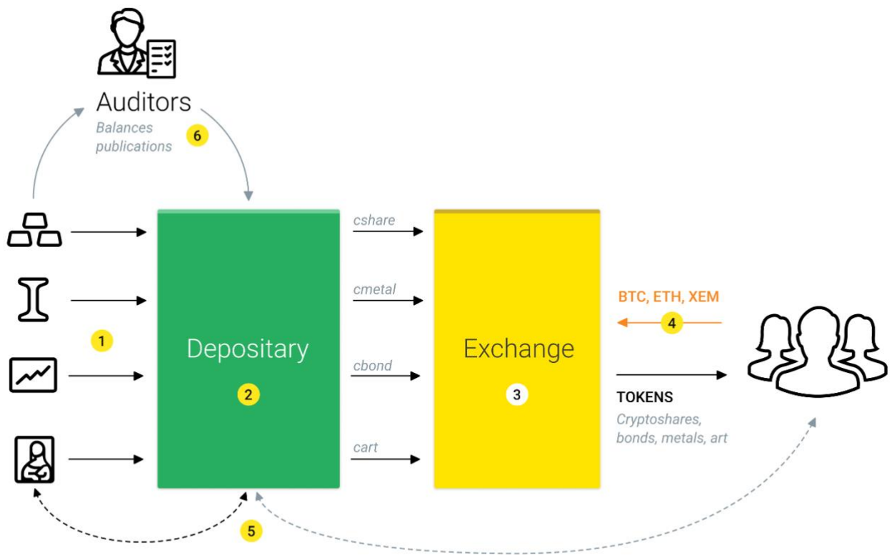
Figure 3. Zeus Depository Workflow.
